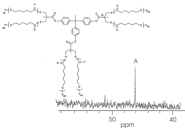
Figure 1. ^{13}\text{C} -NMR spectra of 1a .
