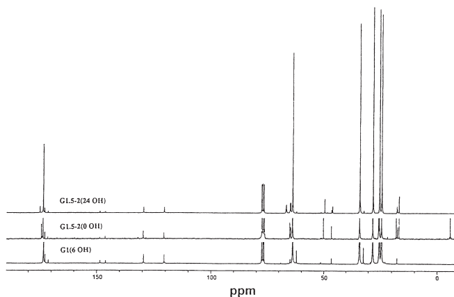
Figure 5. ^{13}\text{C-NMR} spectrum of 15 .
