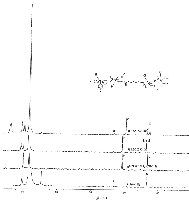
Figure 6. ^{13}\text{C} -NMR spectrum of 15 .
