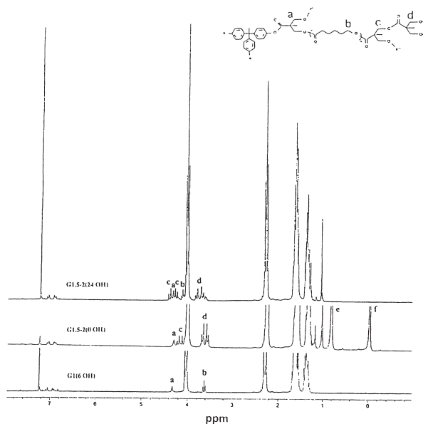
Figure 2. ^1\text{H} -NMR spectra of 1a (bottom), 15 (protected) and 15 (deprotected), top.
